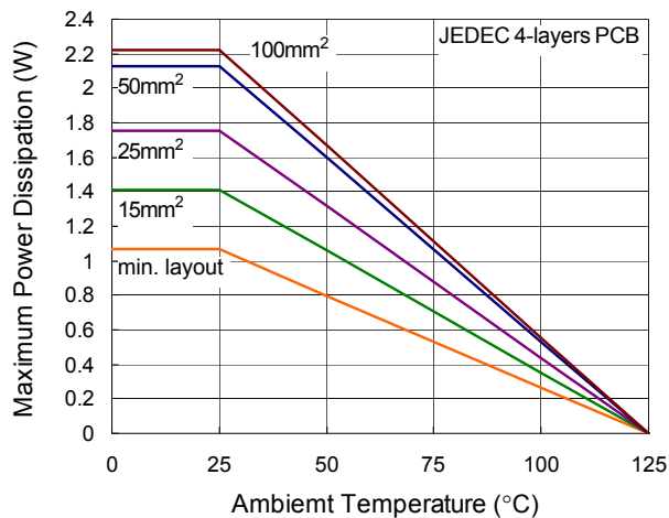
Figure 2. De-rating Curves for RT9027AB Package
